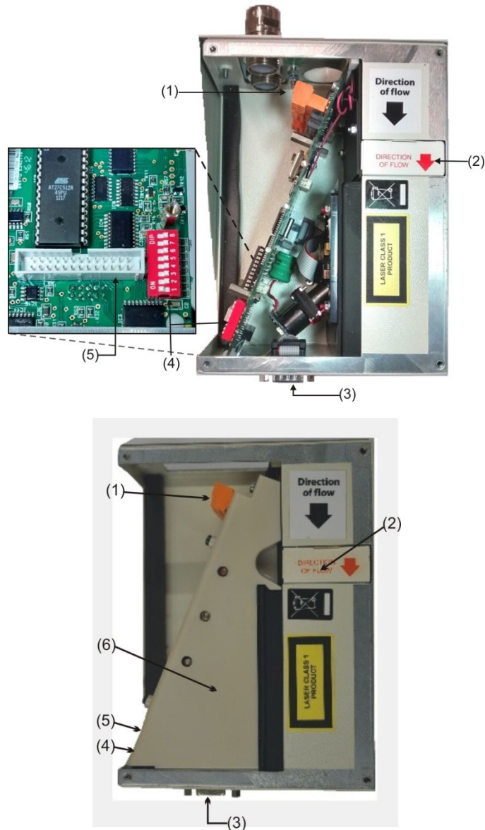
Figure 2: Detector interior view (EN/UL certified models)
