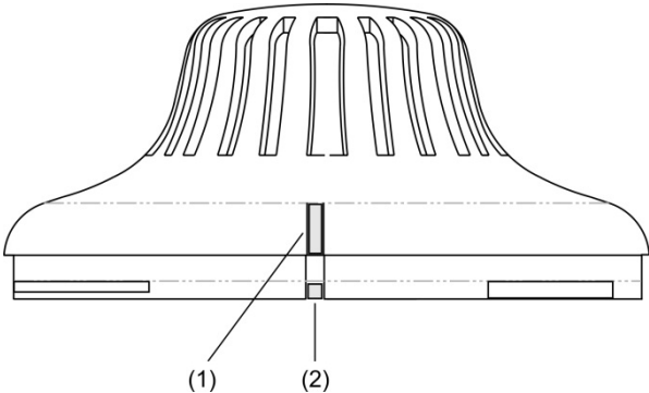
Figure 2: Detector breakout locking tab
