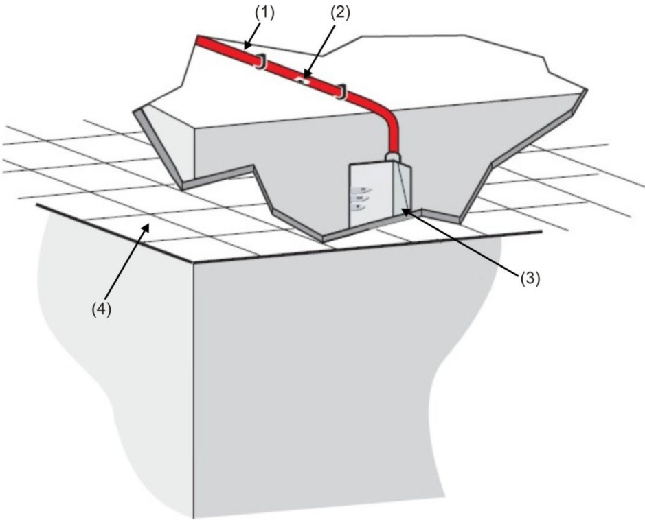
Figure 6: Installation with detector mounted in ceiling void (no exhaust piping)
