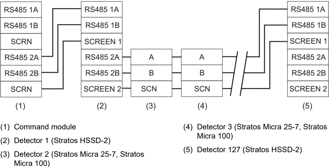
Figure 14: Connecting a detector to a SenseNET network
