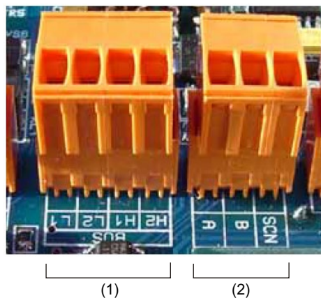
Figure 9: APIC address and RS-485/SenseNET terminals
