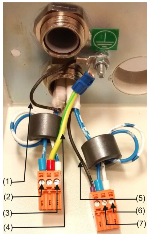
Figure 10: Power and signal connections to the docking station
