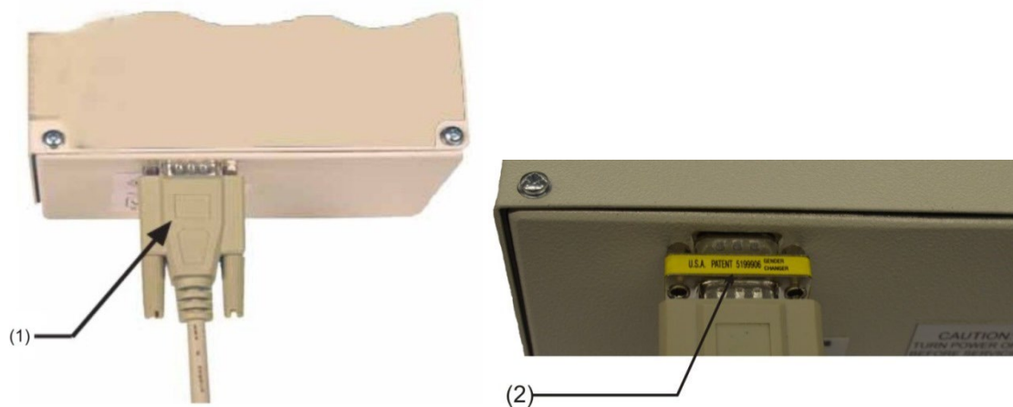
Figure 17: Detector serial port connection for a PC
