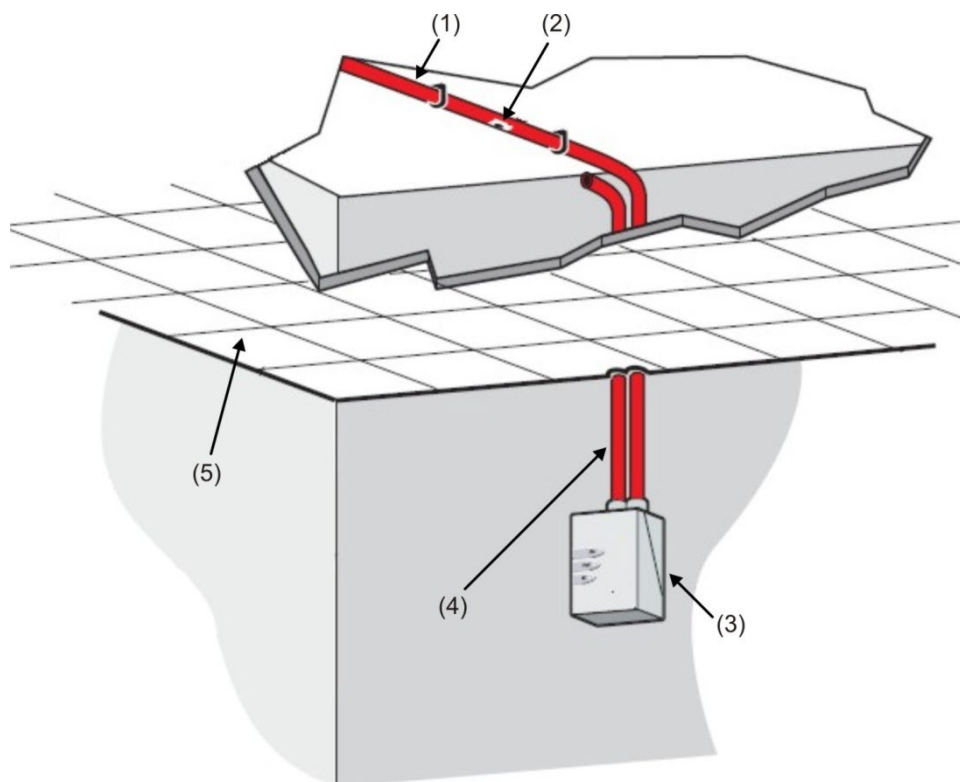
Figure 5: Installation of pipework above ceiling with exposed detector (piped exhaust)
