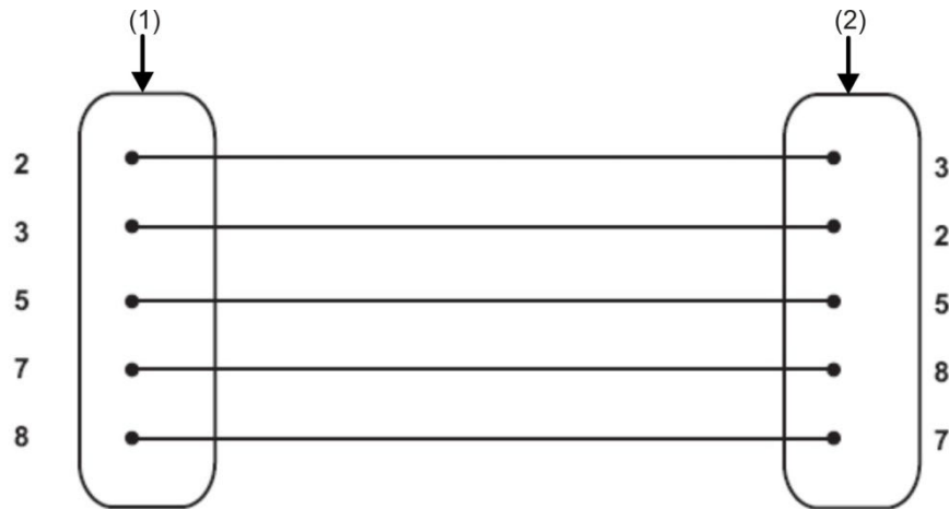
Figure 16: RS-232 cable connections
