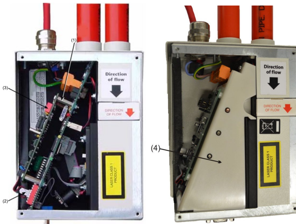
Figure 12: APIC connections (EN/UL certified models)
