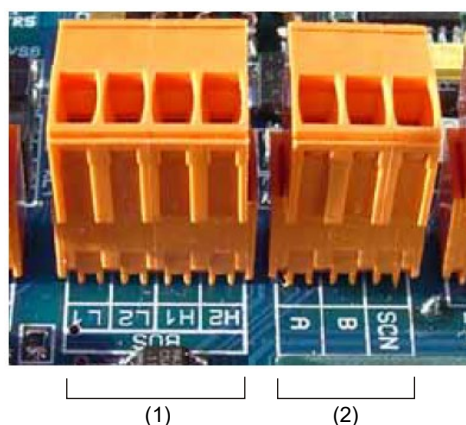
(2) RS-485 / SenseNET terminals
