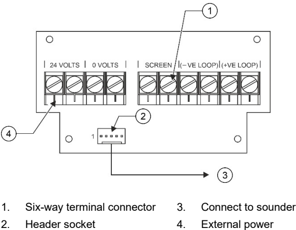
Figure 1: Wiring the PCB
