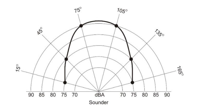
Figure 8: Anechoic sound levels
