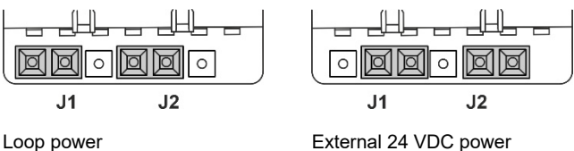
Figure 2: Setting the power source
