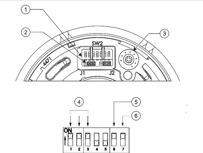
Figure 4: Mode, tone, and volume configuration
