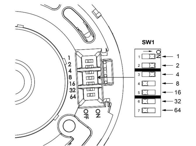
Figure 3: Setting the address
