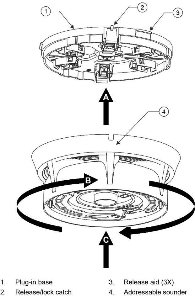
Figure 5: Mounting the sounder
