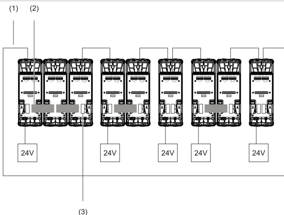
Figure 16 : Cluster hybride
